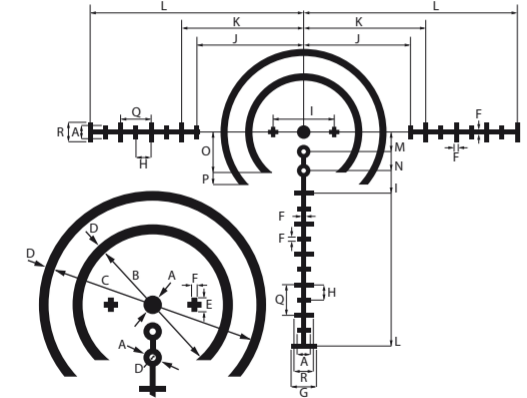
Letters A to R in the diagram above refer to the reticle subtensions of units A to R shown on the table to the right.
